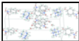
Fig. 1. Thermal ellipsoid plot (Barbour, 2001) of the noncentrosymmetric, triclinic unit-cell contents of C_6H_{12}N_4 \cdot 2C_6H_5NO_3 \cdot H_2O . The probability level is 70%; H-atoms are shown as spheres of arbitrary radius.
